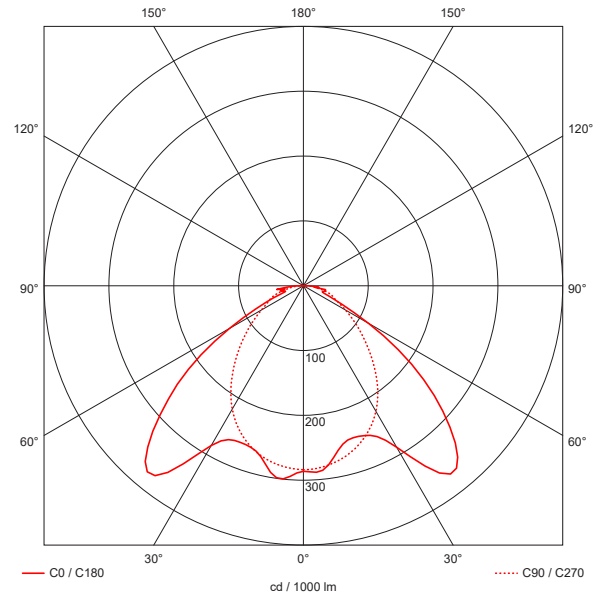
Photometric Diagram
