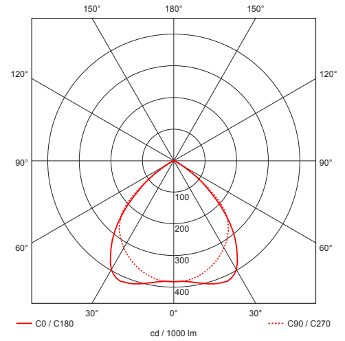
Photometric Diagram
