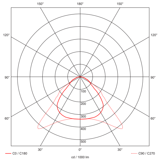
Photometric Diagram
