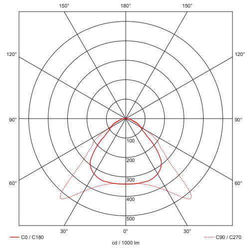
Photometric Diagram
