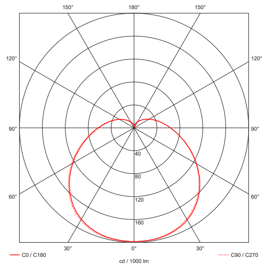
Photometric Diagram
