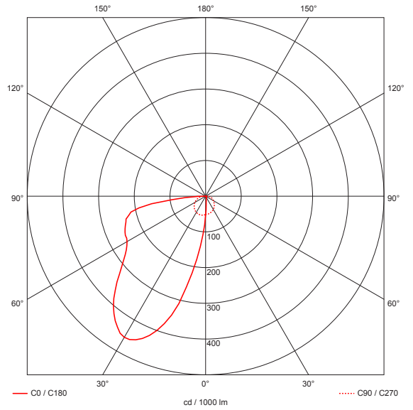
Photometric Diagram
