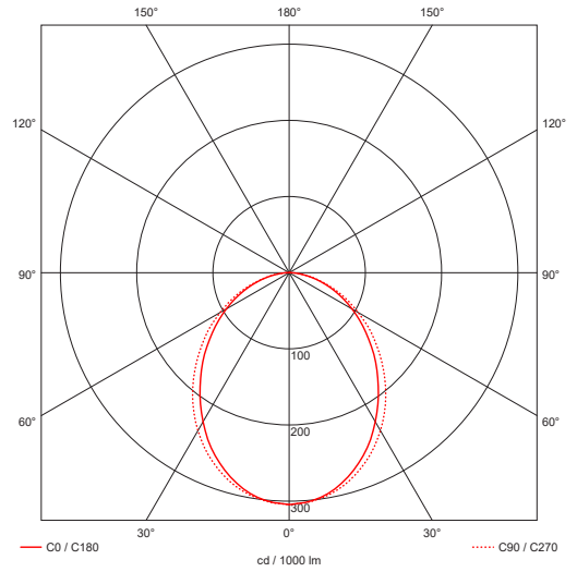
Photometric Diagram
